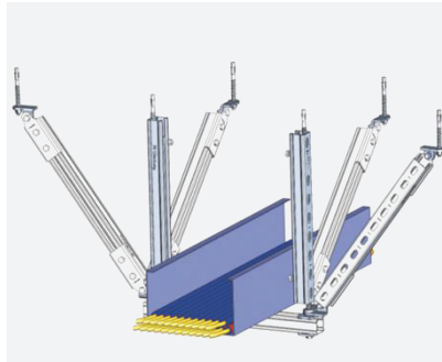
Cable Tray Support (cable box, bus duct)
