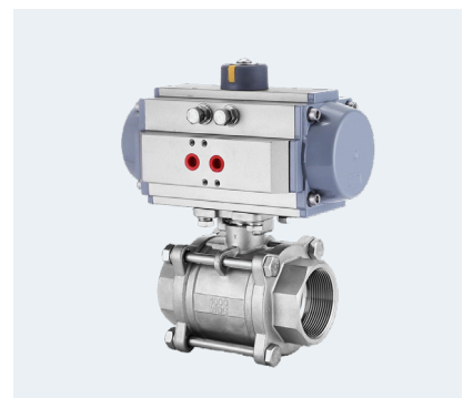
Pneumatic Actuator
